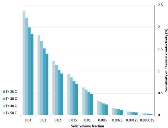
Fig. 8. Sensitivity analysis of thermal conductivity predicted by the experimental model “3” at different temperatures and concentrations
