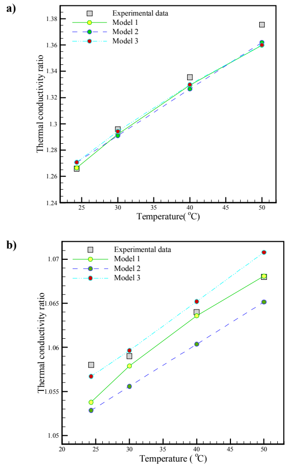
Fig. 4. comparison between experimental data and proposed correlations at a) φ = 5% , b) φ = 1%
