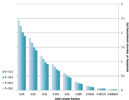
Fig. 7. Sensitivity analysis of thermal conductivity predicted by the experimental model “2” at different temperatures and concentrations
