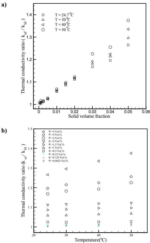
Fig. 3. Thermal conductivity ratio a) at different temperature versus solid volume fraction b) for various concentration with respect to temperature
