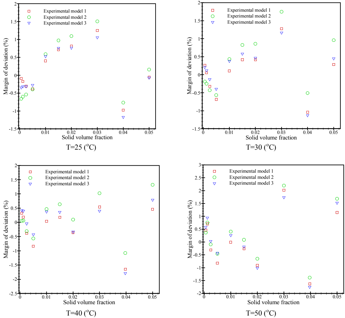
Fig. 5. Margin of deviation for different temperatures
