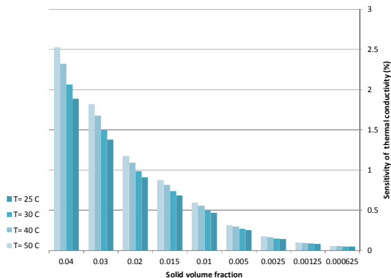
Fig. 6. Sensitivity analysis of thermal conductivity predicted by the experimental model “1” at different temperatures and concentrations
